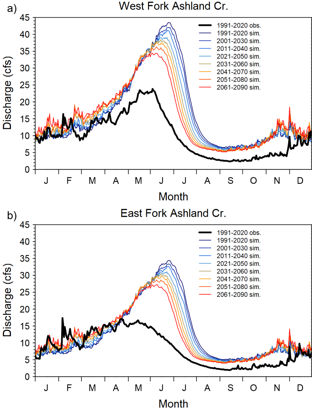
Figure B3. Simulated (sim.) and observed (obs.) 30-year average daily discharge from the a) West Fork and b) East Fork Ashland Creek basins. Simulated discharge is from the LOCA-Hydro5 dataset with the RCP4.5 scenario. LOCA-Hydro5 uses the VIC hydrological model only.
